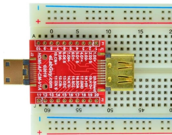
Figure 2: Example of connecting the HDMI-AF-CM-V1A on a proto PCB (Note: This picture only shows the pins spacing, actual use may not be used on a breadboard)
