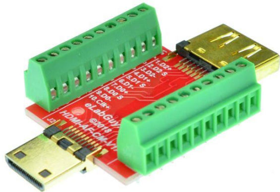
Figure 4: HDMI-AF-CM-V1A with terminal blocks
