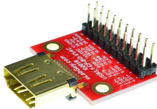
Figure 2: HDMI-AF-BO-V1AC
