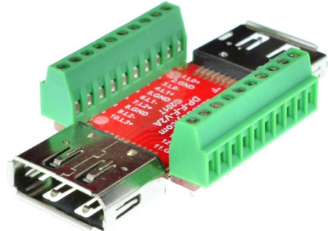
Figure 4: DP-F-F-V2A with terminal blocks
