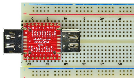
Figure 2: Example of connecting the DP-F-F-V2A on a proto PCB (Note: This picture only shows the pins spacing, actual use may not be used on a breadboard)
