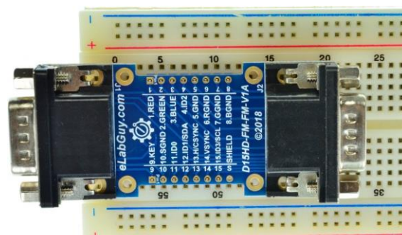
Figure 2: Example of connecting the D15HD-M-M-V1A on a proto PCB (Note: This picture only shows the pins spacing, actual use may not be used on a breadboard)
