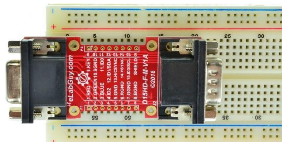
Figure 2: Example of connecting the D15HD-F-M-V1A on a proto PCB (Note: This picture only shows the pins spacing, actual use may not be used on a breadboard)
