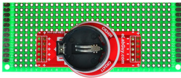
Figure 4: Solid Mounting on prototype PCB
