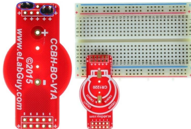
Figure 5: side way connection
