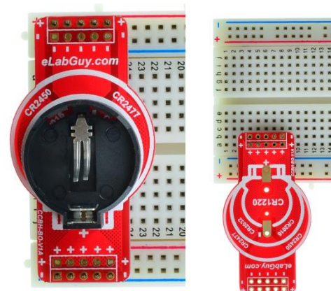
Figure 2: Example of connecting the CR2032-BO-V1A on breadboard
