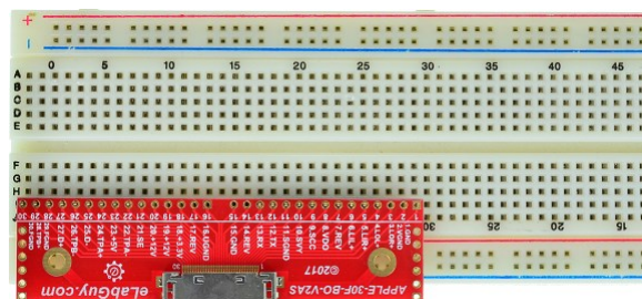
Figure 2: Example of connecting the APPLE-30F-BO-V2AS on a breadboard
