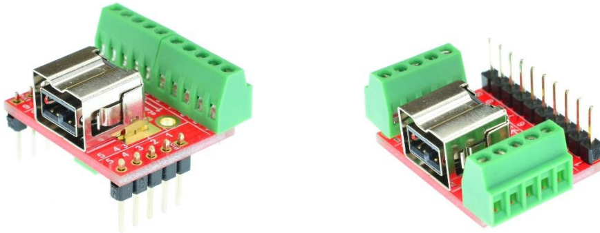
Figure 3: 1394-9F-BO-V1A Various connections
