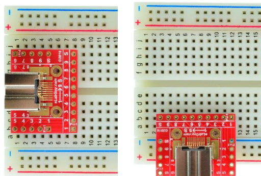
Figure 2: Example of connecting the 1394-9F-BO-V1A on a breadboard
