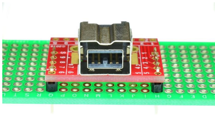
Figure 5: Solid Mounting on prototype PCB
