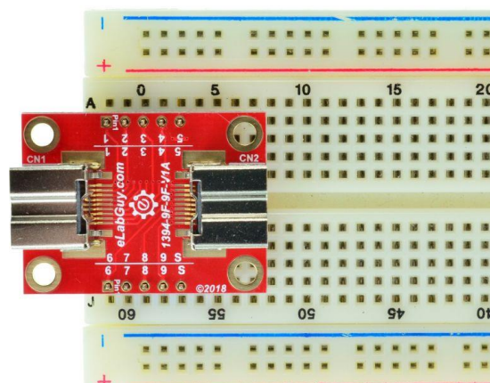
Figure 2: Example of connecting the 1394-9F-9F-V1A on a proto PCB (Note: This picture only shows the pins spacing, actual use may not be used on a breadboard)
